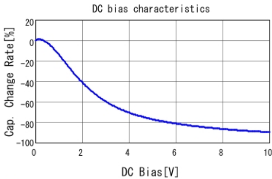
■ GRT155R61A225KE01 C-DC bias capchange, 25.0degC, AC0.
