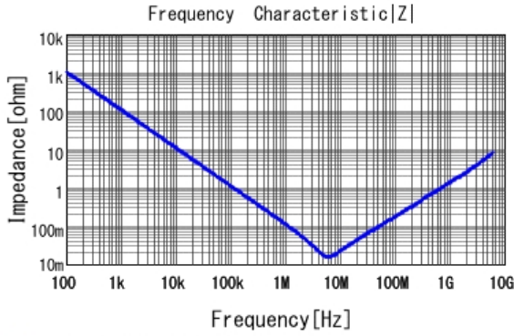
■ GRT155R61A225KE01 |Z| DC0V, 25degC
