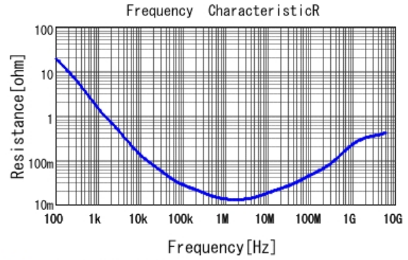
■ GRT155R61A225KE01 R DC0V, 25degC
