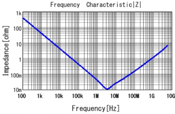
■ GRT155R61A475ME13 |Z| DCOV, 25degC
