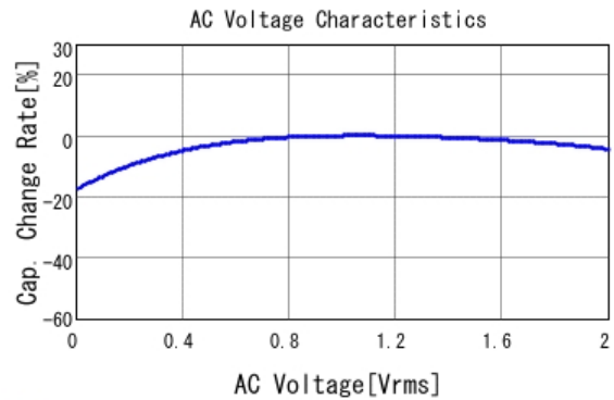
■ GRT155R61A475ME13 C-AC Voltage capchange, DCOV, 25.0d
