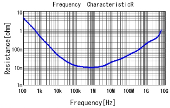
■ GRT155R61A475ME13 R DCOV, 25degC
