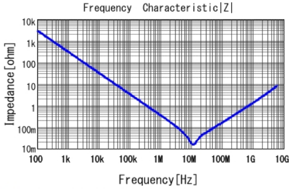
■ GRT155R61C105KE01 |Z| DC0V, 25degC
