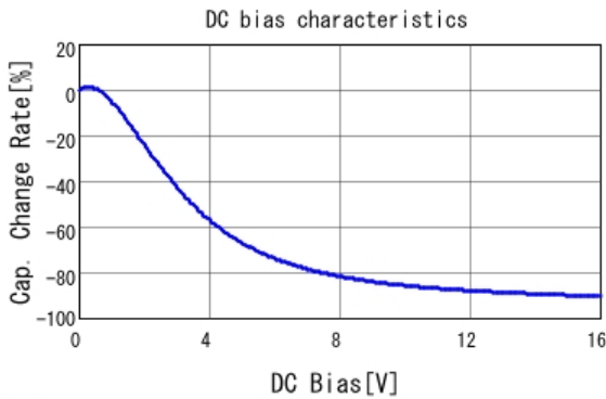
■ GRT155R61C105KE01 C-DC bias capchange, 25.0degC, AC1.
