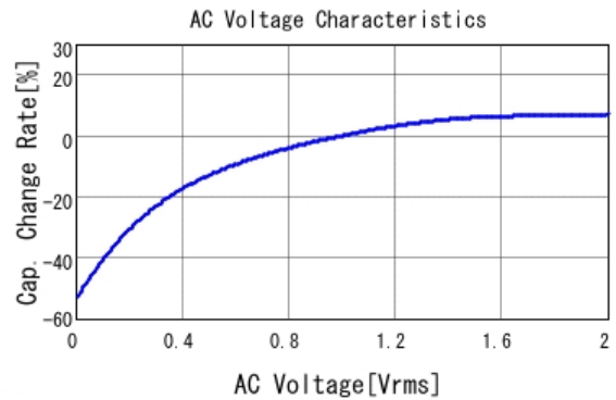
■ GRT155R61C105KE01 C-AC Voltage capchange, DC0V, 25.0d
