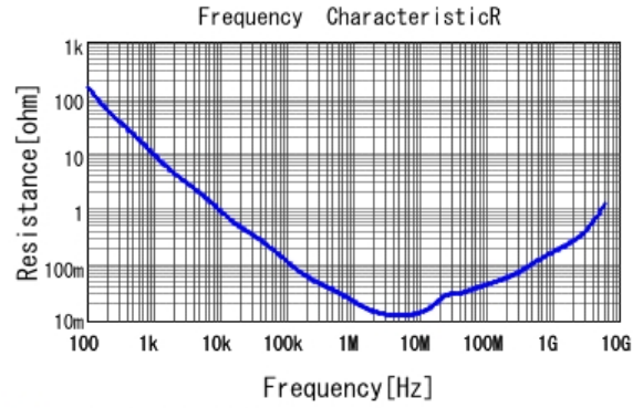
■ GRT155R61C105KE01 R DC0V, 25degC
