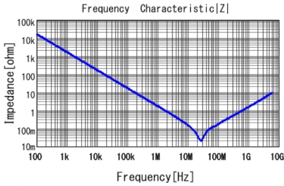
■ GRT155R71C104KE01 |Z| DC0V, 25degC
