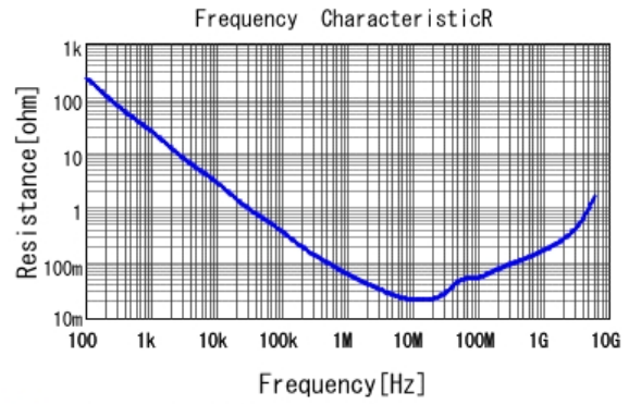
■ GRT155R71C224KE01 R DC0V, 25degC
