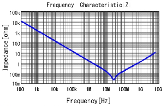
■ GRT155R71C224KE01 |Z| DC0V, 25degC
