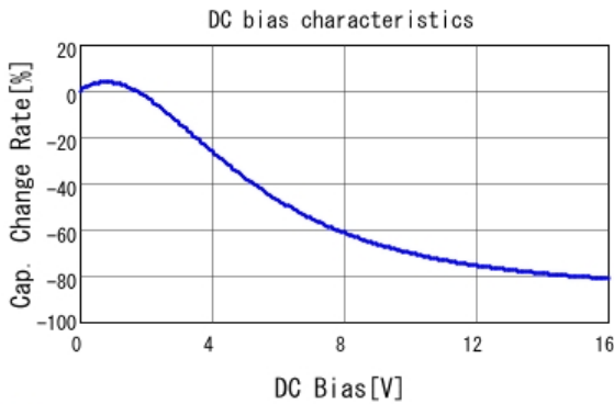
■ GRT155R71C224KE01 C-DC bias capchange, 25.0degC, AC1.
