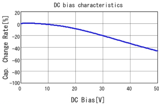
■ GRT155R71H103KE01 C-DC bias capchange, 25.0degC, AC1.
