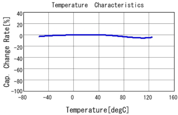
■ GRT155R71H103KE01 C-Temp. capchange, DC0.0V, AC1.0Vrm
