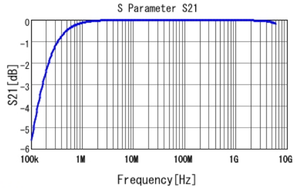
■ GRT155R71H103KE01 S21 DC0V, 25degC
