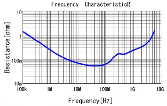
■ GRT155R71H103KE01 R DCOV, 25degC
