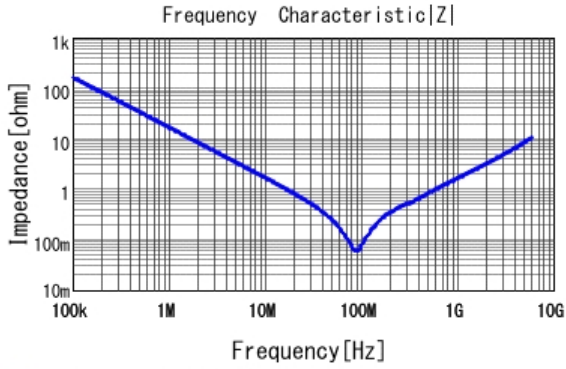
■ GRT155R71H103KE01 |Z| DCOV, 25degC
