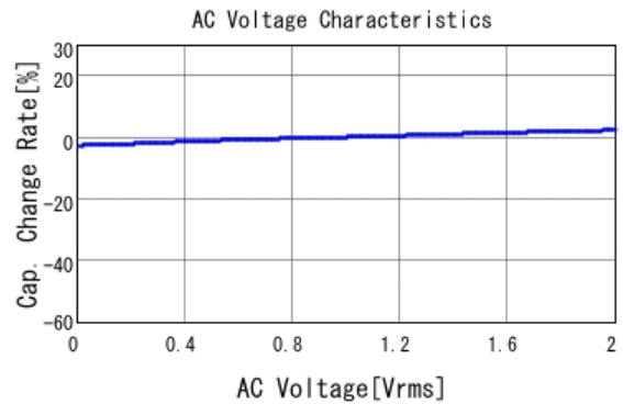
■ GRT155R71H103KE01 C-AC Voltage capchange, DCOV, 25.0d
