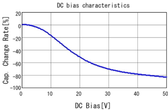
■ GRT155R71H104KE01 C-DC bias capchange, 25.0degC, AC1.
