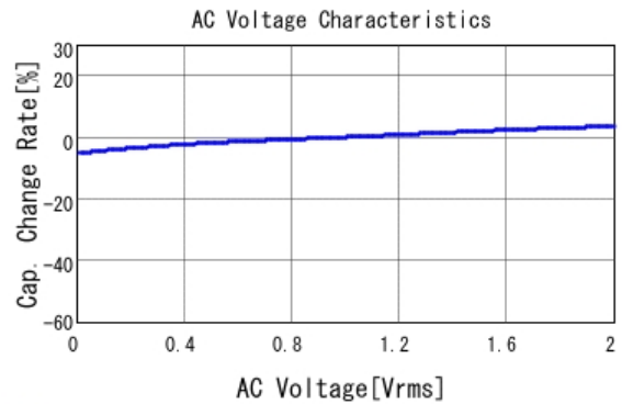
■ GRT155R71H104KE01 C-AC Voltage capchange, DC0V, 25.0d
