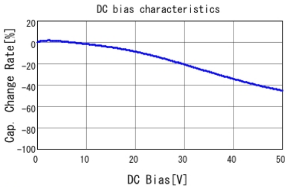
■ GRT155R71H152KE01 C-DC bias capchange, 25.0degC, AC1.
