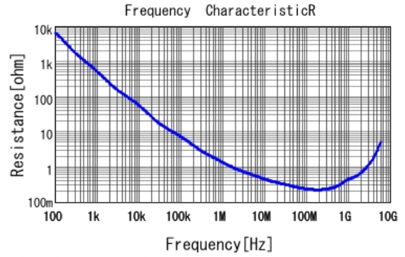
■ GRT155R71H152KE01 R DCOV, 25degC
