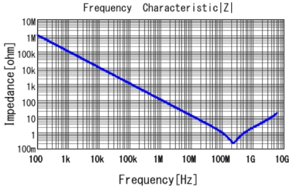
■ GRT155R71H152KE01 |Z| DCOV, 25degC
