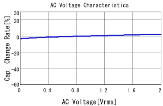
■ GRT155R71H152KE01 C-AC Voltage capchange, DCOV, 25.0d
