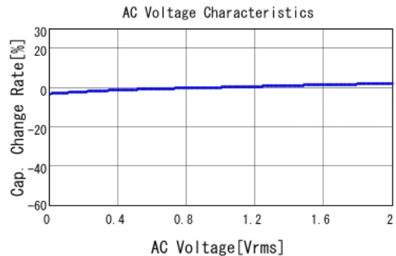
■ GRT155R71H222KE01 C-AC Voltage capchange, DCOV, 25.0d
