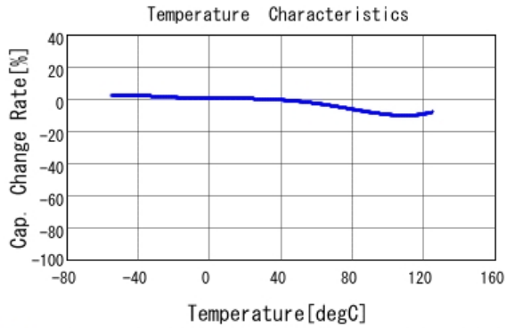
■ GRT155R71H222KE01 C-Temp. capchange, DC0.0V, AC1.0Vrm
