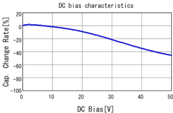
■ GRT155R71H222KE01 C-DC bias capchange, 25.0degC, AC1.
