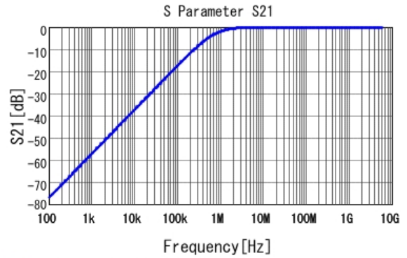
■ GRT155R71H222KE01 S21 DC0V, 25degC
