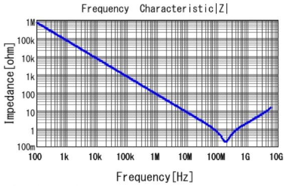
■ GRT155R71H222KE01 |Z| DCOV, 25degC
