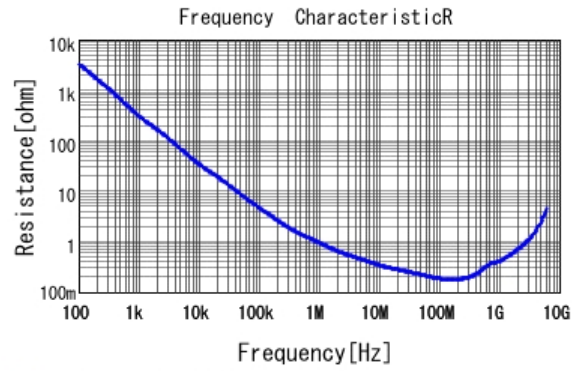
■ GRT155R71H222KE01 R DCOV, 25degC
