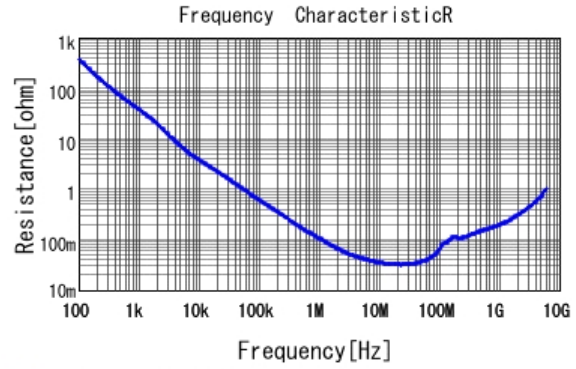
■ GRT155R71H223KE01 R DC0V, 25degC
