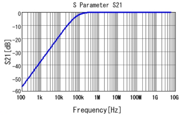
■ GRT155R71H223KE01 S21 DC0V, 25degC
