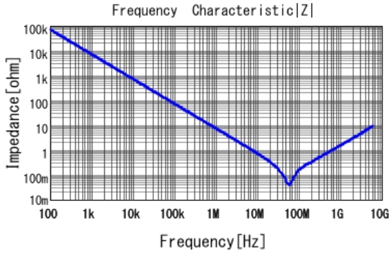
■ GRT155R71H223KE01 |Z| DC0V, 25degC
