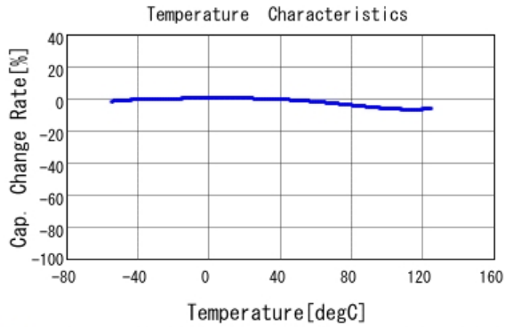
■ GRT155R71H223KE01 C-Temp. capchange, DC0.0V, AC1.0Vrm
