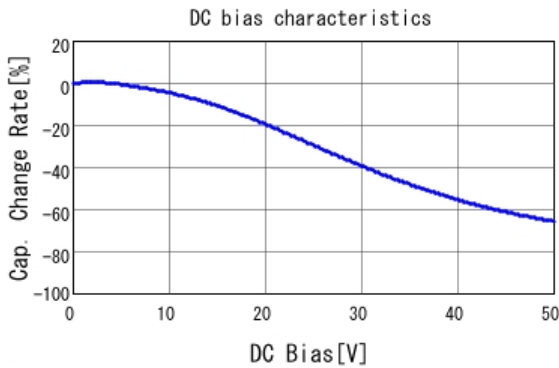
■ GRT155R71H223KE01 C-DC bias capchange, 25.0degC, AC1.
