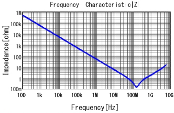
■ GRT155R71H332KE01 |Z| DCOV, 25degC
