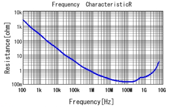
■ GRT155R71H332KE01 R DCOV, 25degC
