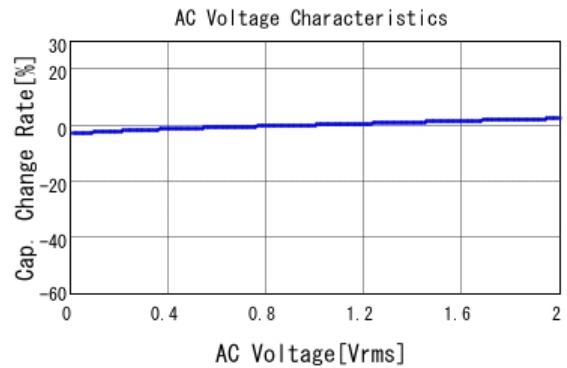
■ GRT155R71H332KE01 C-AC Voltage capchange, DCOV, 25.0d
