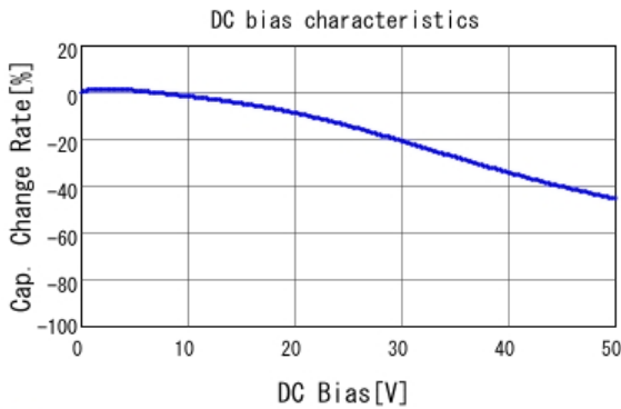
■ GRT155R71H332KE01 C-DC bias capchange, 25.0degC, AC1.
