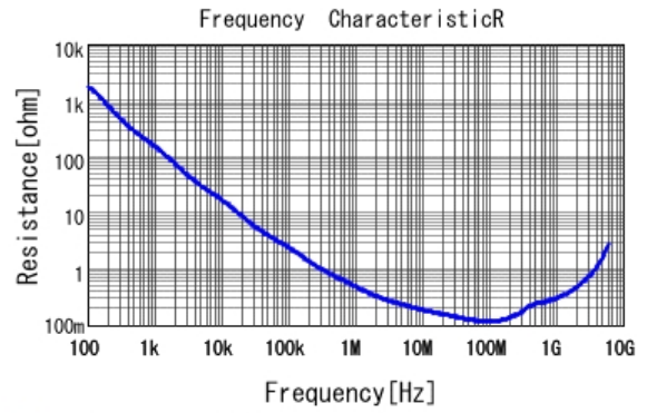
■ GRT155R71H472KE01 R DCOV, 25degC
