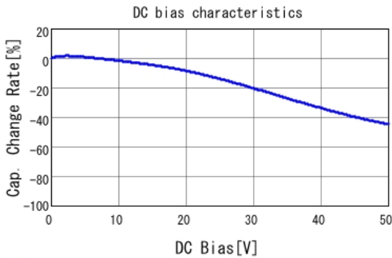
■ GRT155R71H472KE01 C-DC bias capchange, 25.0degC, AC1.
