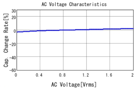
■ GRT155R71H472KE01 C-AC Voltage capchange, DCOV, 25.0d
