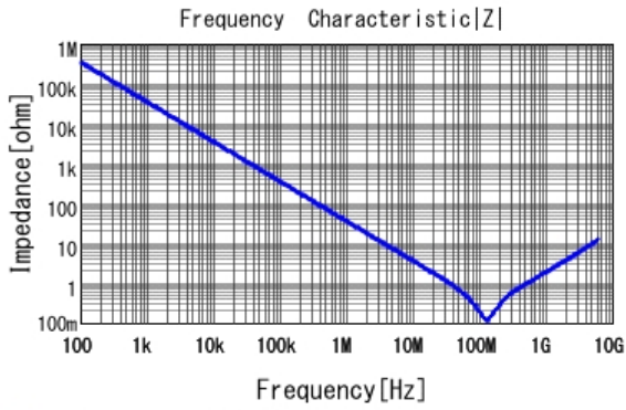
■ GRT155R71H472KE01 |Z| DCOV, 25degC
