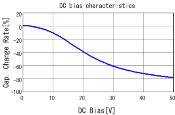
■ GRT155R71H473KE01 C-DC bias capchange, 25.0degC, AC1.
