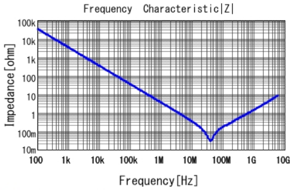
■ GRT155R71H473KE01 |Z| DC0V, 25degC
