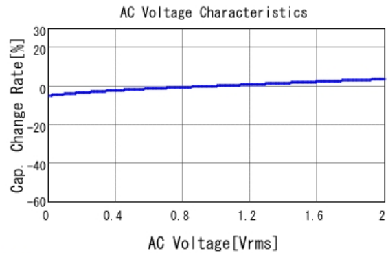
■ GRT155R71H473KE01 C-AC Voltage capchange, DC0V, 25.0d
