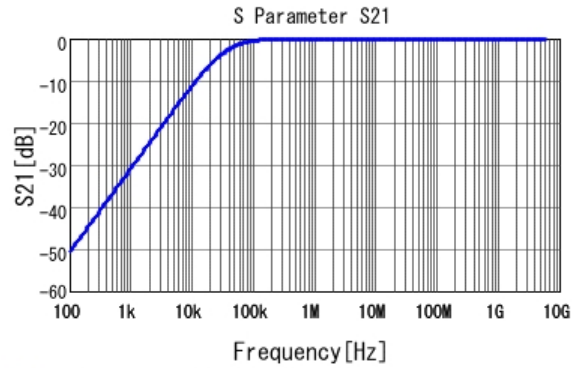
■ GRT155R71H473KE01 S21 DC0V, 25degC
