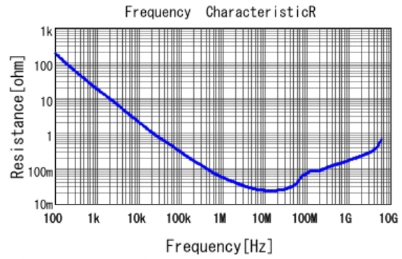
■ GRT155R71H473KE01 R DC0V, 25degC
