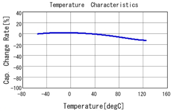
■ GRT155R71H473KE01 C-Temp. capchange, DC0.0V, AC1.0Vrm
