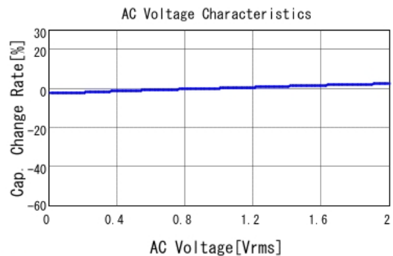
■ GRT155R71H682KE01 C-AC Voltage capchange, DCOV, 25.0d
