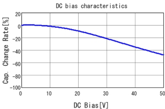
■ GRT155R71H682KE01 C-DC bias capchange, 25.0degC, AC1.
