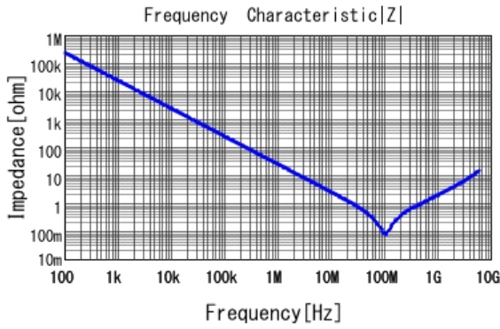
■ GRT155R71H682KE01 |Z| DCOV, 25degC
