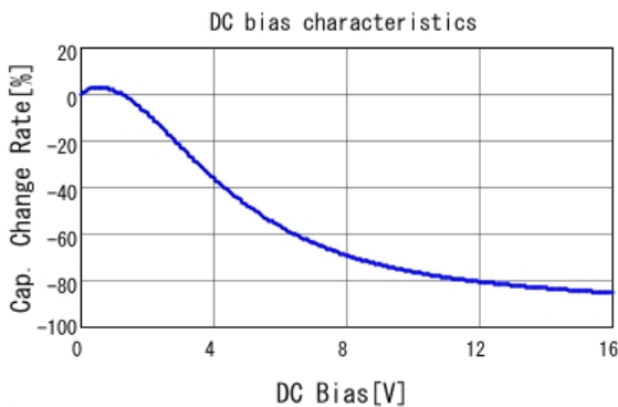
■ GRT188C81C225KE13 C-DC bias capchange, 25.0degC, AC1.
