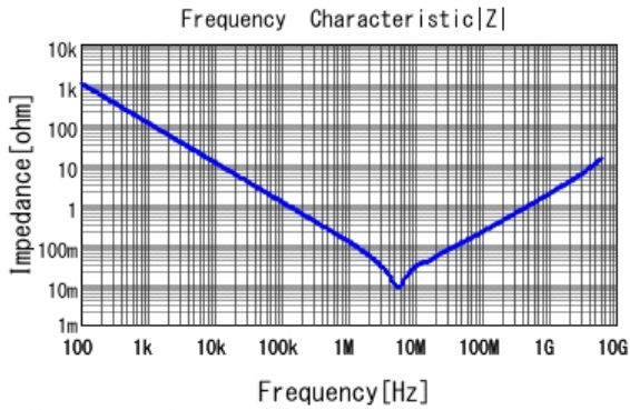
■ GRT188C81C225KE13 |Z| DCOV, 25degC
