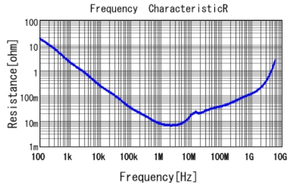
■ GRT188C81C225KE13 R DCOV, 25degC
