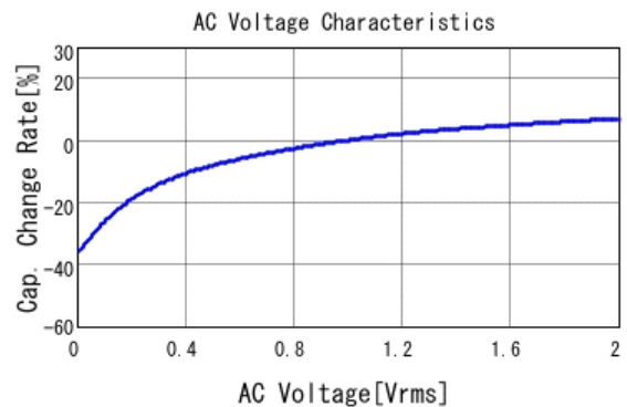
■ GRT188C81C225KE13 C-AC Voltage capchange, DCOV, 25.0d
