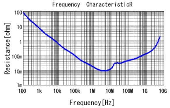
■ GRT188C8YA105KE13 R DCOV, 25degC
