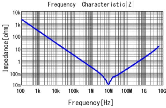
■ GRT188C8YA105KE13 |Z| DCOV, 25degC
