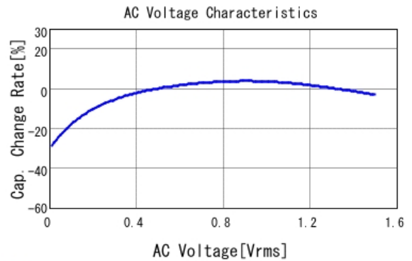
■ GRT188R60J226ME13 C-AC Voltage capchange, DCOV, 25.0d
