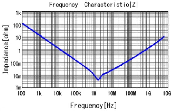
■ GRT188R60J226ME13 |Z| DCOV, 25degC
