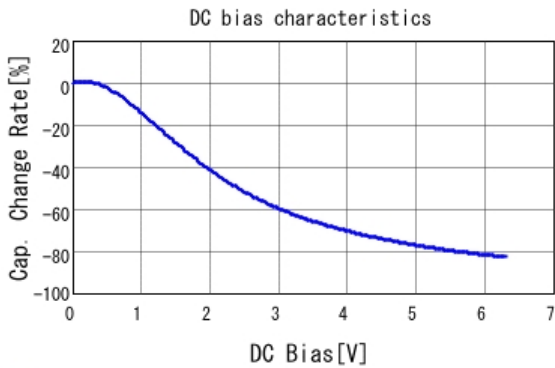
■ GRT188R60J226ME13 C-DC bias capchange, 25.0degC, AC0.
