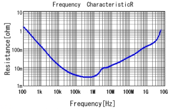
■ GRT188R60J226ME13 R DCOV, 25degC
