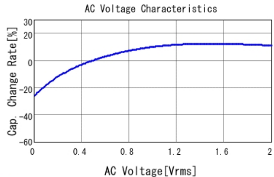
■ GRT188R60J475KE01 C-AC Voltage capchange, DCOV, 25.0d
