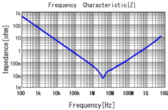
■ GRT188R60J475KE01 |Z| DCOV, 25degC
