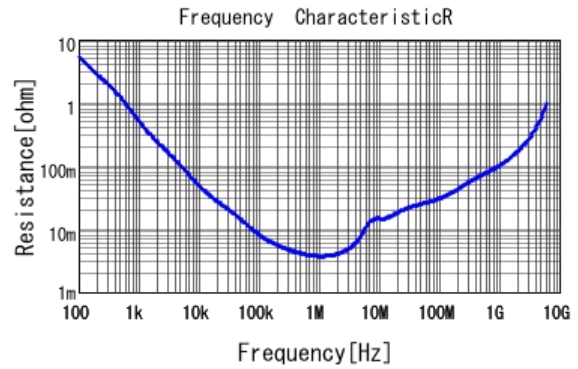
■ GRT188R60J475KE01 R DCOV, 25degC
