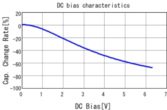
■ GRT188R60J475KE01 C-DC bias capchange, 25.0degC, AC0.
