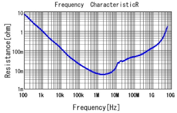
■ GRT188R61A105KE01 R DCOV, 25degC
