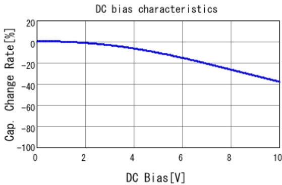
■ GRT188R61A105KE01 C-DC bias capchange, 25.0degC, AC1.
