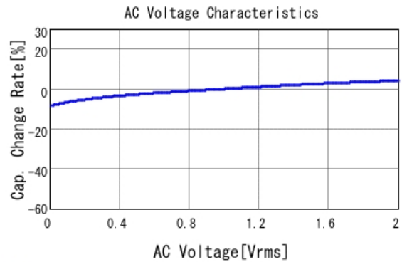
■ GRT188R61A105KE01 C-AC Voltage capchange, DCOV, 25.0d
