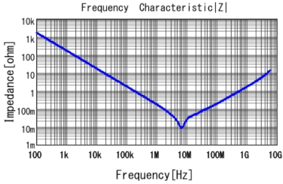
■ GRT188R61A105KE01 |Z| DCOV, 25degC
