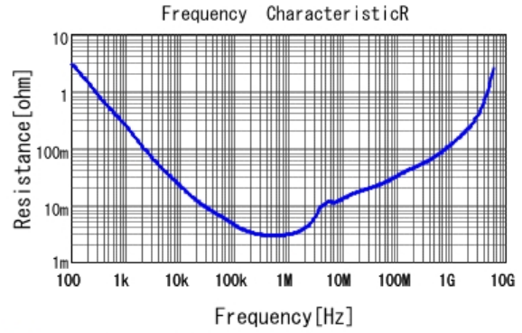
■ GRT188R61A106KE13 R DCOV, 25degC
