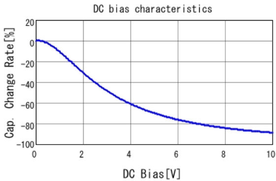
■ GRT188R61A106KE13 C-DC bias capchange, 25.0degC, AC0.
