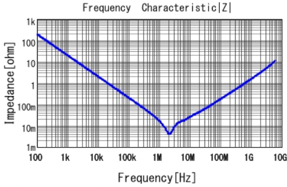
■ GRT188R61A106KE13 |Z| DCOV, 25degC
