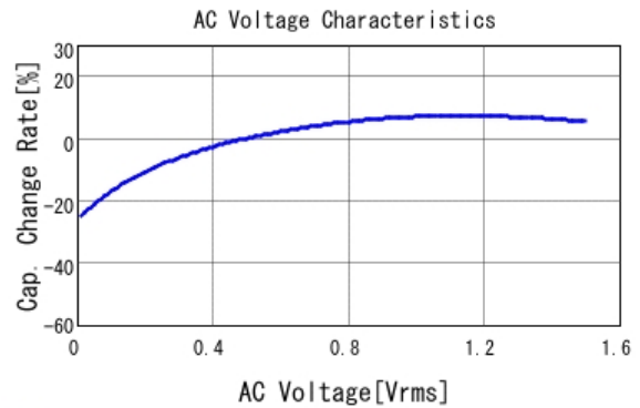
■ GRT188R61A106KE13 C-AC Voltage capchange, DCOV, 25.0d
