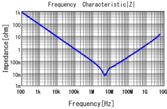
■ GRT188R61A225KE13 |Z| DCOV, 25degC
