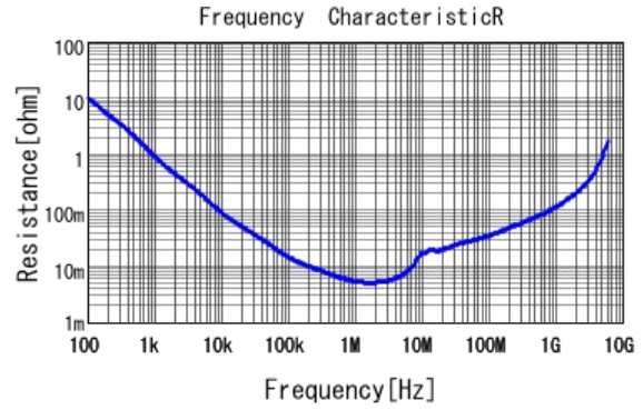
■ GRT188R61A225KE13 R DCOV, 25degC
