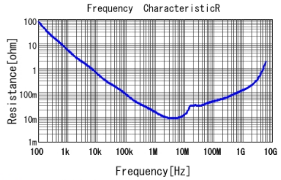
■ GRT188R61E105KE13 R DCOV, 25degC
