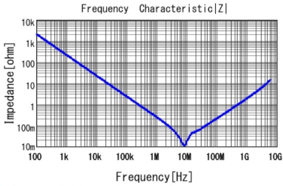
■ GRT188R61E105KE13 |Z| DCOV, 25degC
