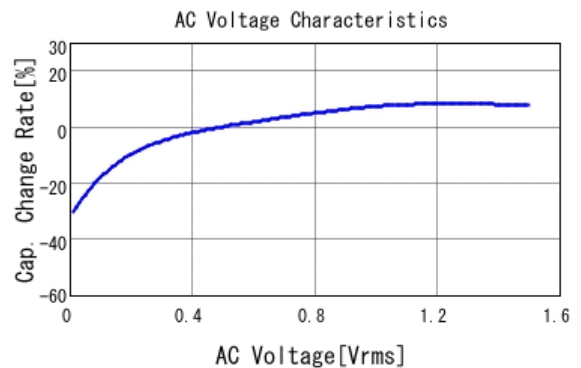
■ GRT21BR60J226ME13 C-AC Voltage capchange, DCOV, 25.0d
