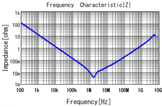
■ GRT21BR60J226ME13 |Z| DCOV, 25degC
