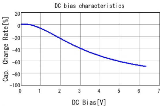
■ GRT21BR60J226ME13 C-DC bias capchange, 25.0degC, AC0.
