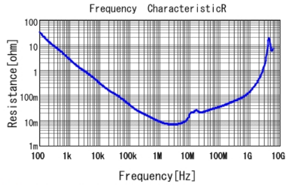
■ GRT21BR61H225KE13 R DCOV, 25degC
