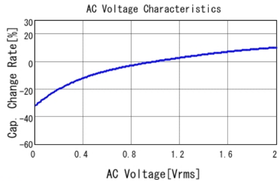
■ GRT21BR61H225KE13 C-AC Voltage capchange, DCOV, 25.0d
