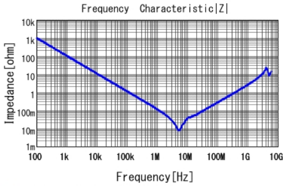
■ GRT21BR61H225KE13 |Z| DCOV, 25degC
