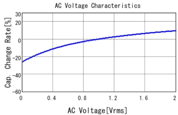
■ GRT21BR71E225KE13 C-AC Voltage capchange, DC0V, 25.0d
