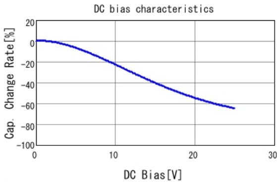
■ GRT21BR71E225KE13 C-DC bias capchange, 25.0degC, AC1.
