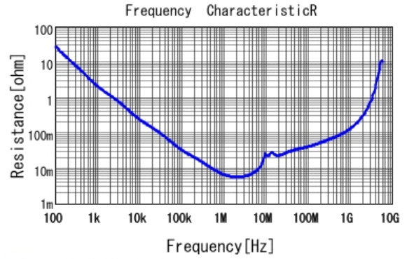
■ GRT21BR71E225KE13 R DC0V, 25degC
