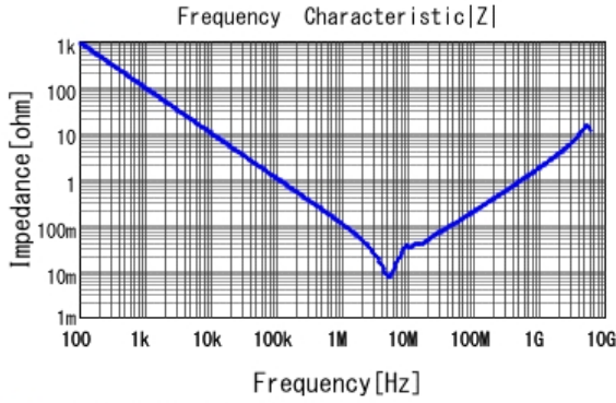
■ GRT21BR71E225KE13 |Z| DC0V, 25degC
