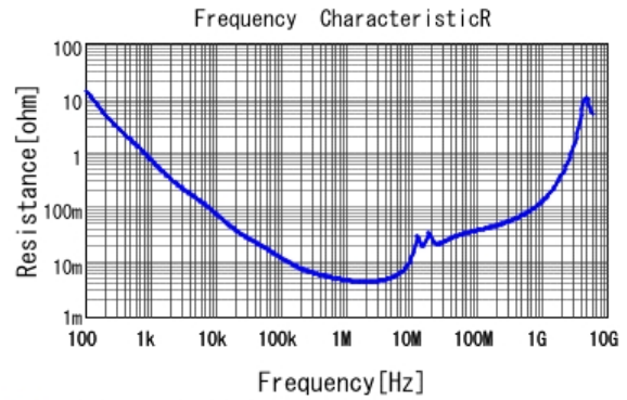
■ GRT21BR71H105KE01 R DC0V, 25degC
