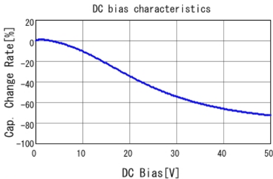
■ GRT21BR71H105KE01 C-DC bias capchange, 25.0degC, AC1.
