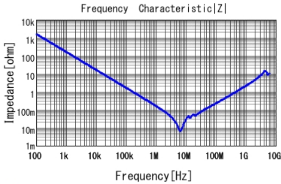
■ GRT21BR71H105KE01 |Z| DC0V, 25degC
