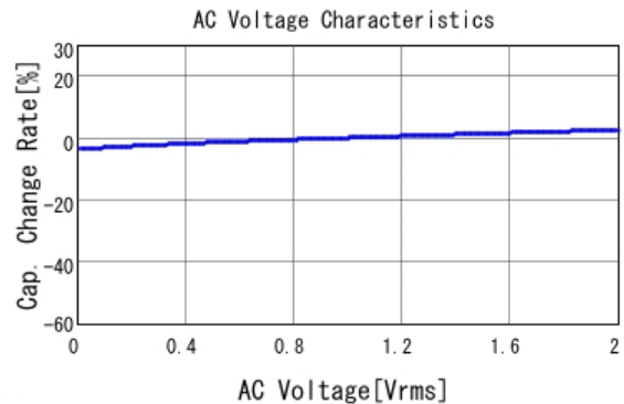
■ GRT21BR71H105KE01 C-AC Voltage capchange, DC0V, 25.0d
