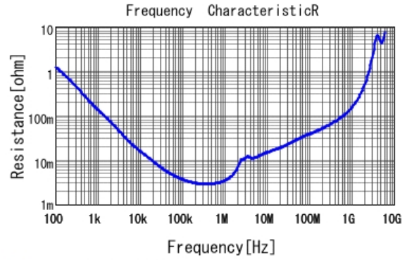
■ GRT31CC81C226KE01 R DCOV, 25degC
