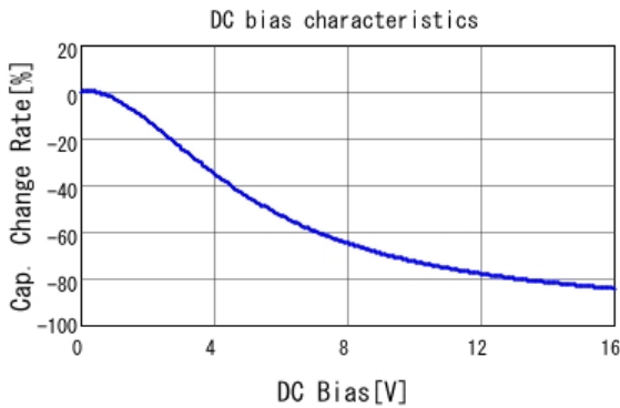
■ GRT31CC81C226KE01 C-DC bias capchange, 25.0degC, AC0.
