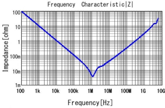
■ GRT31CC81C226KE01 |Z| DCOV, 25degC
