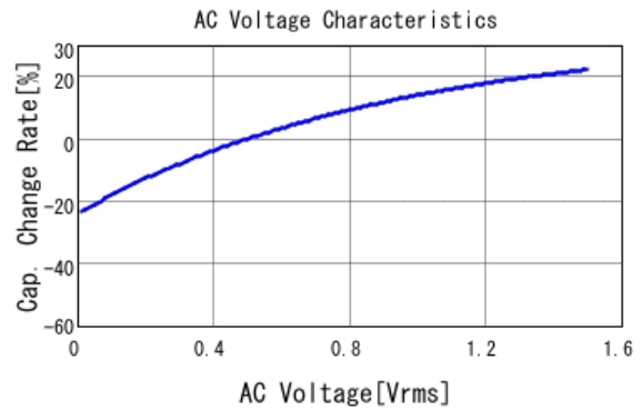
■ GRT31CC81C226KE01 C-AC Voltage capchange, DCOV, 25.0d
