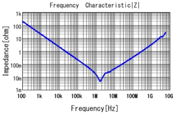
■ GRT31CC81E106KE01 |Z| DC0V, 25degC
