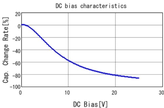
■ GRT31CC81E106KE01 C-DC bias capchange, 25.0degC, AC1.
