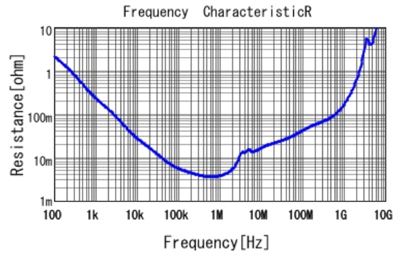
■ GRT31CC81E106KE01 R DC0V, 25degC
