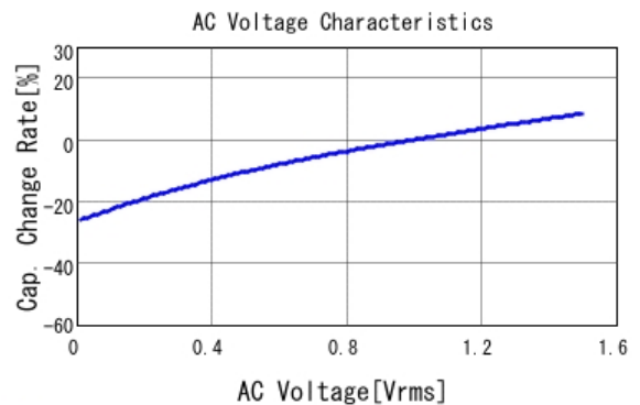
■ GRT31CC81E106KE01 C-AC Voltage capchange, DC0V, 25.0d
