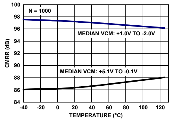
FIGURE 20. CMRR vs TEMPERATURE, V_{CM} = +1.0V \text{ TO } -2.0V, +5.1V \text{ TO } -0.1V
