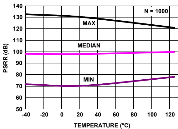
FIGURE 21. PSRR vs TEMPERATURE, V_+, V_- = \pm 0.9V \text{ TO } \pm 2.5V
