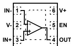
ISL28194 (6 LD 1.6X1.6X0.5 UTDFN) TOP VIEW
