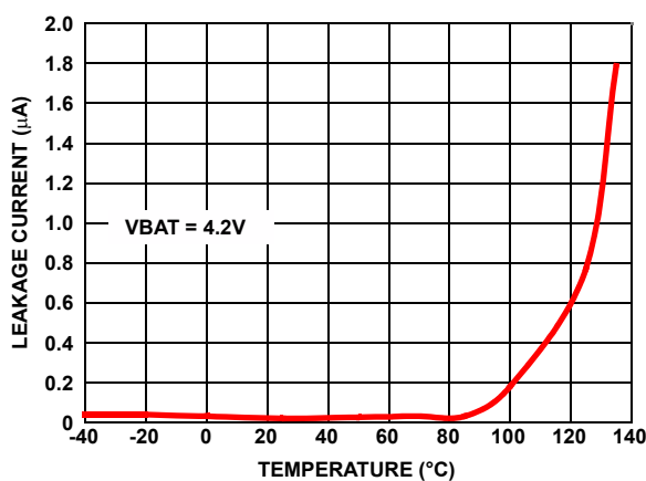
FIGURE 6. REVERSE CURRENT vs TEMPERATURE
