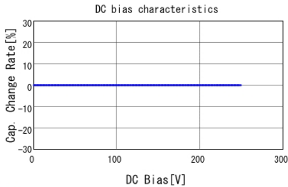
■ KCA55L7UMF332KH01 C-DC bias capchange, 25.0degC, AC1V
