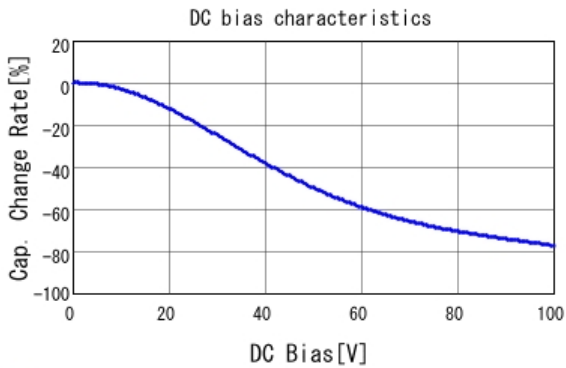
■ KCM55QR72A106KH01 C-DC bias capchange, 25.0degC, AC1V
