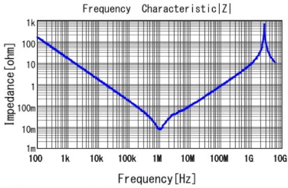
■ KCM55QR72A106KH01 |Z| DC0V, 25degC
