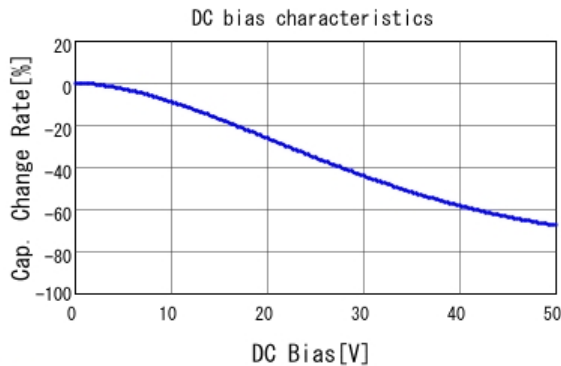
■ KRM31KR71H225KH01 C-DC bias capchange, 25.0degC, AC1V
