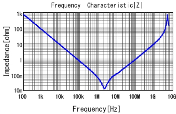
■ KRM31KR71H225KH01 |Z| DC0V, 25degC
