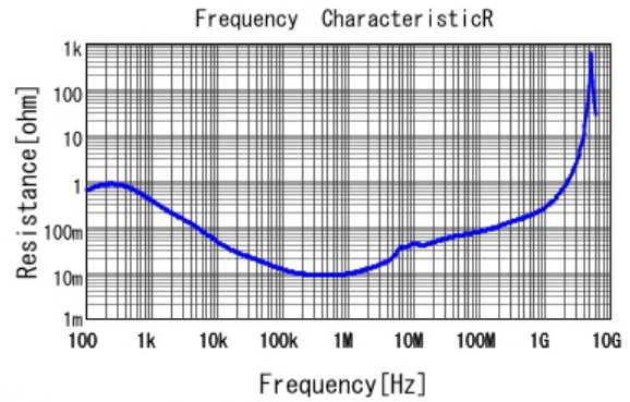
■ KRM31KR71H225KH01 R DC0V, 25degC
