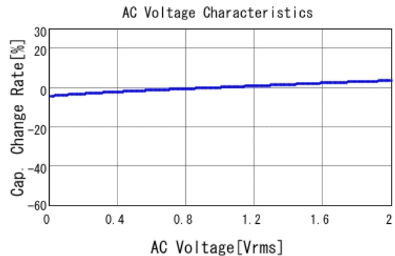
■ KRM31KR71H225KH01 C-AC Voltage capchange, DC0V, 25.0d
