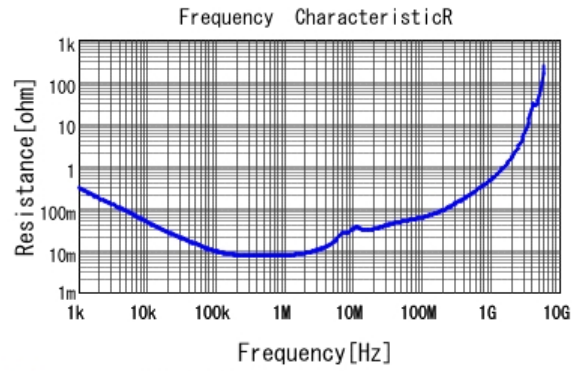
■ KRM31KR72A225KH01 R DC0V, 25degC
