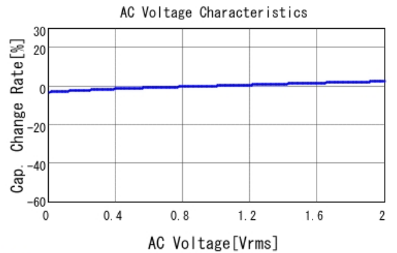
■ KRM31KR72A225KH01 C-AC Voltage capchange, DC0V, 25.0d
