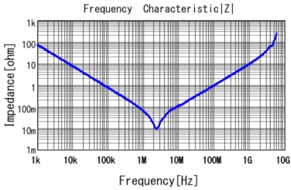
■ KRM31KR72A225KH01 |Z| DC0V, 25degC
