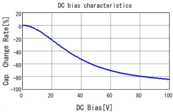
■ KRM31KR72A225KH01 C-DC bias capchange, 25.0degC, AC1V
