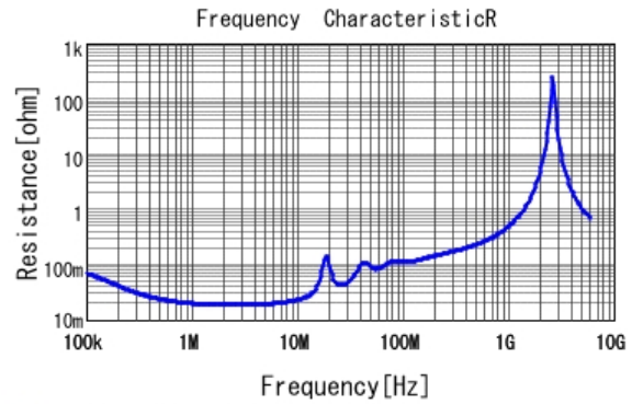
■ KRM55TR73A224MH01 R DC0V, 25degC
