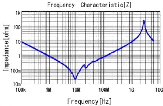
■ KRM55TR73A224MH01 |Z| DC0V, 25degC
