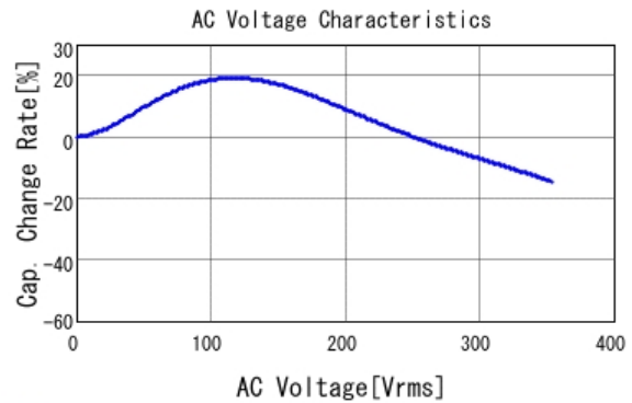
■ KRM55TR73A224MH01 C-AC Voltage capchange, DC0V, 25.0d
