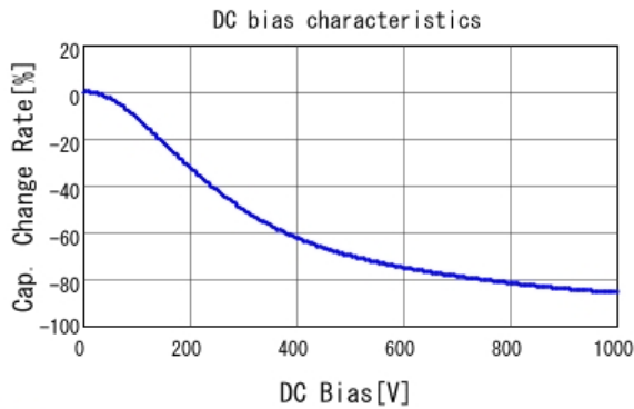
■ KRM55TR73A224MH01 C-DC bias capchange, 25.0degC, AC1V
