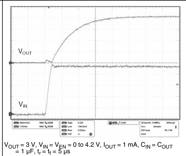
Figure 30. Startup transient
