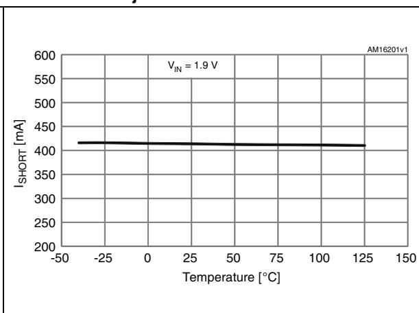
Figure 10. Short-circuit current vs. temp. for adjustable version
