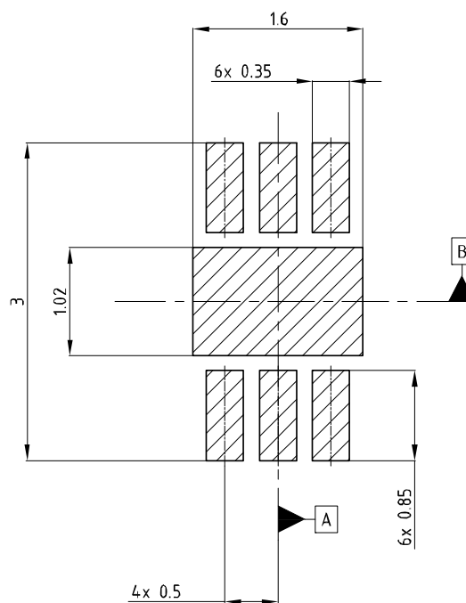
Figure 32: DFN (2x2) recommended footprint
