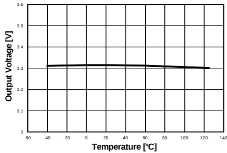
Figure 5: Output voltage vs temperature ( V_{OUT} = 3.3 V , I_{OUT} = 5 mA )
