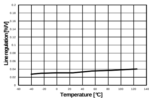
Figure 9: Line regulation vs temperature
