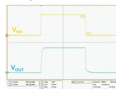
Figure 26: Turn-on time
