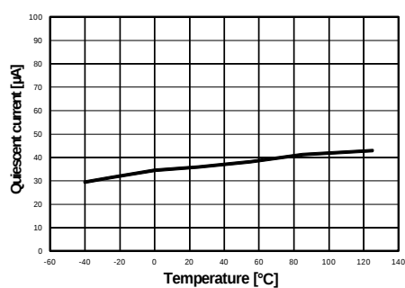
Figure 11: Quiescent current vs temperature ( I_{OUT} = 0 \text{ mA} )
