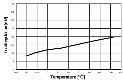
Figure 10: Load regulation vs temperature
