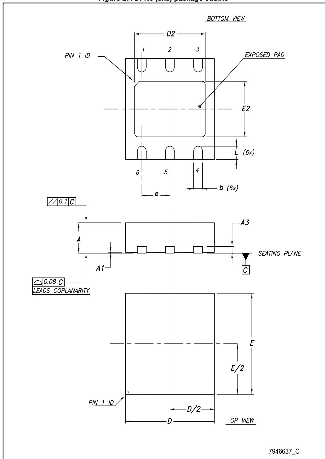
Figure 27: DFN6 (3x3) package outline
