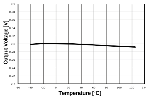
Figure 7: Output voltage vs temperature ( V_{OUT} = V_{ADJ} , I_{OUT} = 5 mA )
