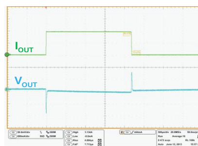
Figure 24: Load transient
