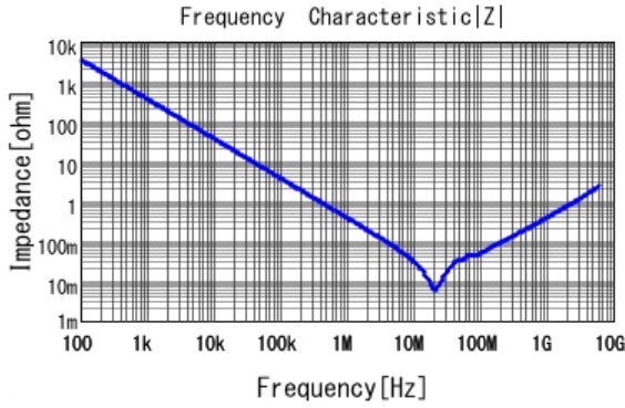
■ LLL153C70G474ME17 |Z| DCOV, 25degC
