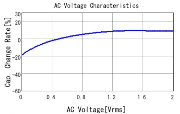
■ LLL153C70G474ME17 C-AC Voltage capchange, DCOV, 25.0d
