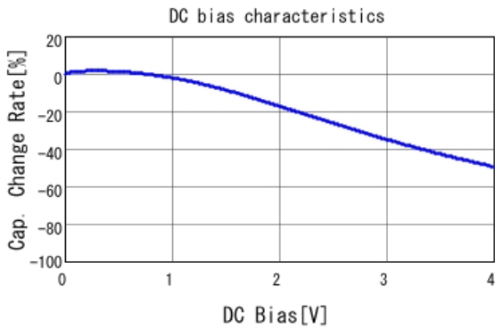
■ LLL153C70G474ME17 C-DC bias capchange, 25.0degC, AC0.
