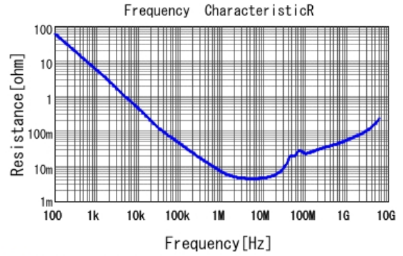
■ LLL153C70G474ME17 R DCOV, 25degC
