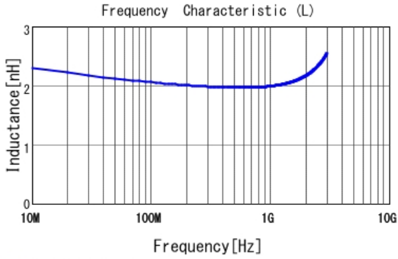
■ LQG15HH2N0S02 L
