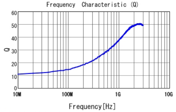
■ LQG15HH2N0S02 Q
