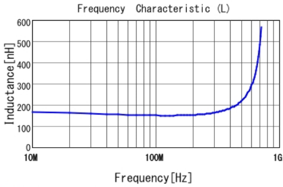
■ LQG15HHR15G02 L
