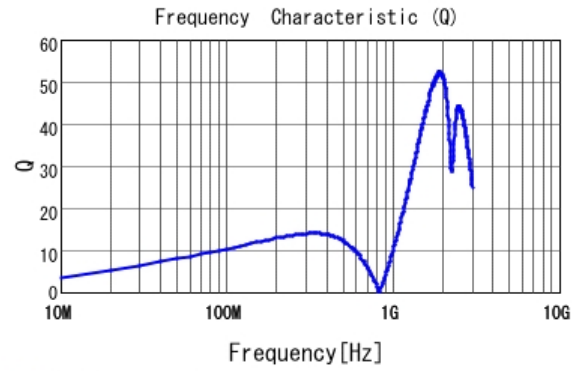
■ LQG15HHR15G02 Q
