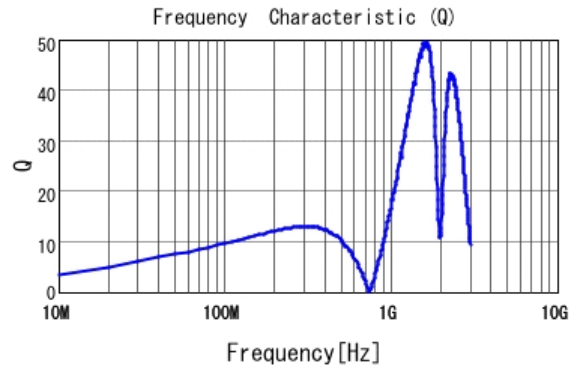
■ LQG15HHR18J02 Q
