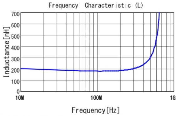
■ LQG15HHR18J02 L
