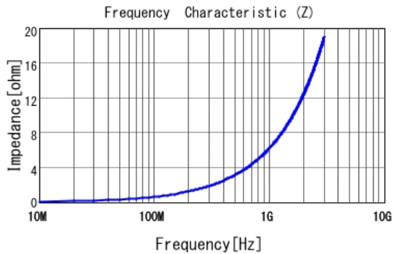
■ LQG15HN1N0S02 |Z|
