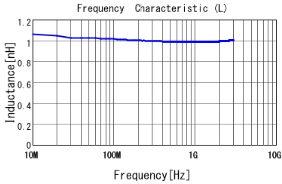
■ LQG15HN1N0S02 L
