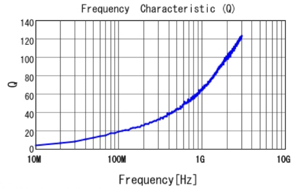
■ LQG15HN1N0S02 Q
