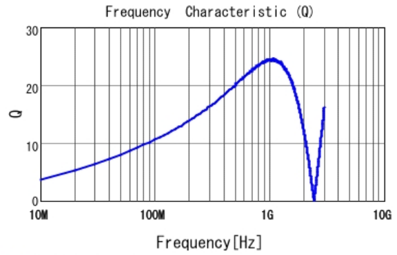
■ LQG15HN22NJ02 Q
