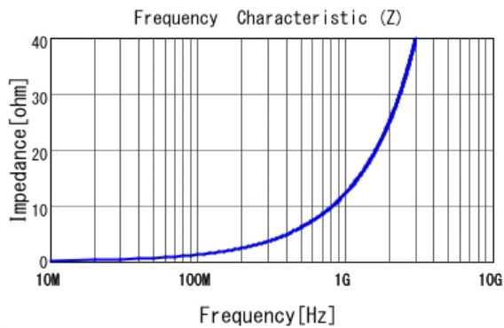
■ LQG15HN2N0S02 |Z|
