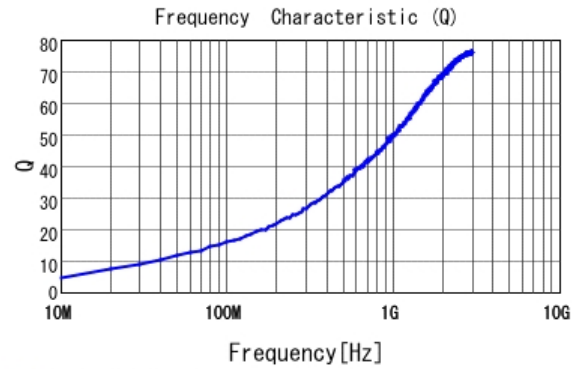
■ LQG15HN2N0S02 Q
