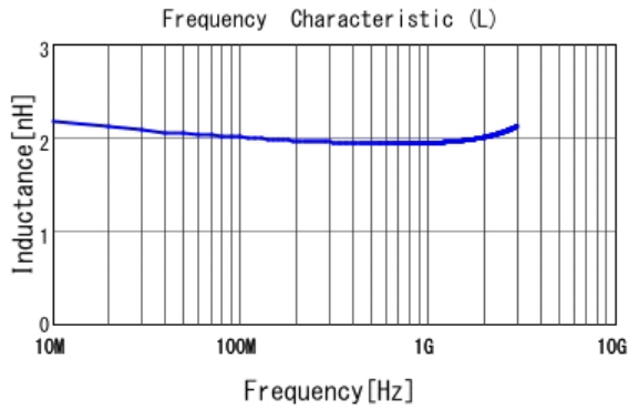
■ LQG15HN2N0S02 L
