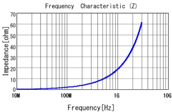
■ LQG15HN3N0S02 |Z|
