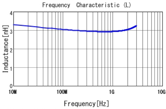
■ LQG15HN3N0S02 L
