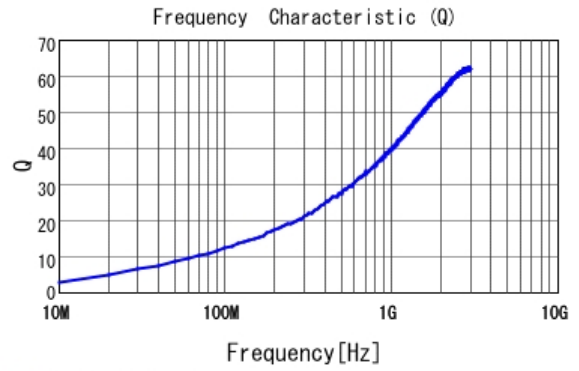
■ LQG15HN3N0S02 Q
