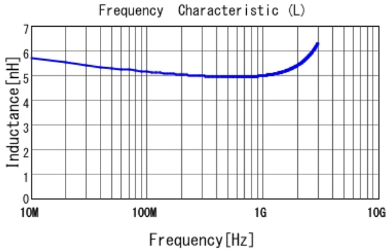
■ LQG15HN5N1S02 L
