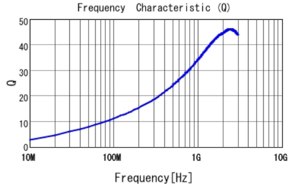
■ LQG15HN5N1S02 Q
