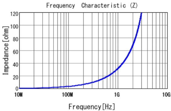
■ LQG15HN5N1S02 |Z|
