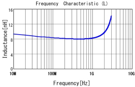
■ LQG15HN8N2J02 L
