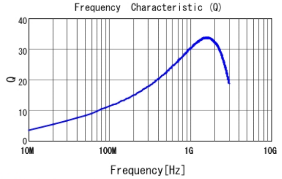
■ LQG15HN9N1J02 Q
