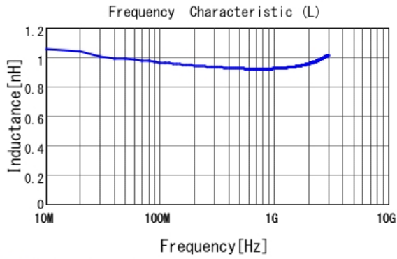
■ LQG15HS1N0B02 L
