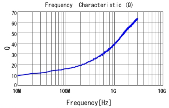
■ LQG15HS1N0B02 Q
