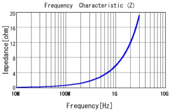
■ LQG15HS1N0S02 |Z|
